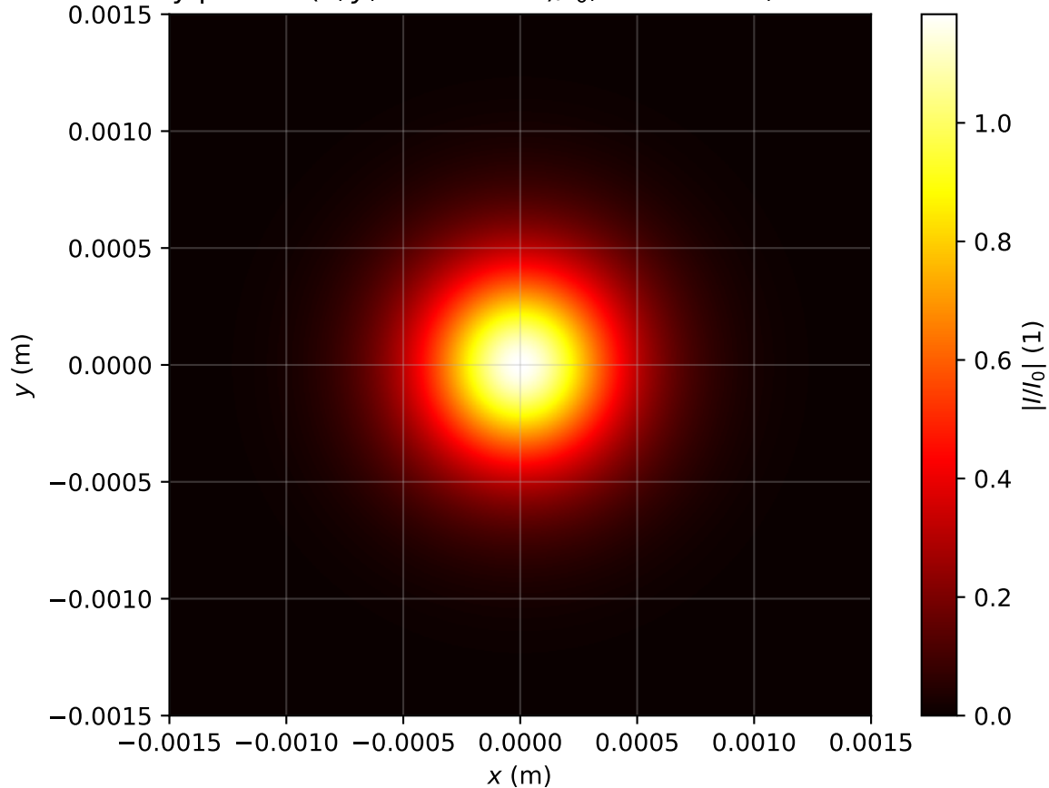
Intensity profile I(x, y, z = 0.876m)/I_0 , P_{in}=0.7P_{cr} , artificial time
